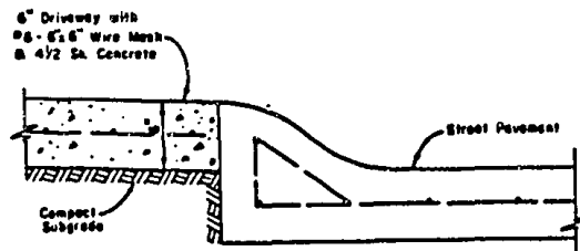
PARTIAL SECTION
