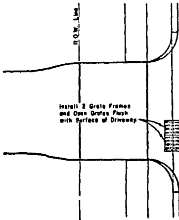
INLET IN DRIVEWAY
