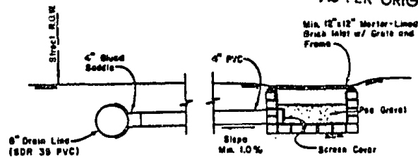
SIDE - LOT DRAIN LINES
