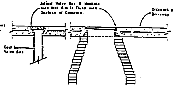
WATER VALVE BOX AND MANHOLE IN SIDEWALK OR DRIVEWAY
