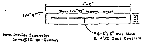
CONCRETE SIDEWALK DETAIL
