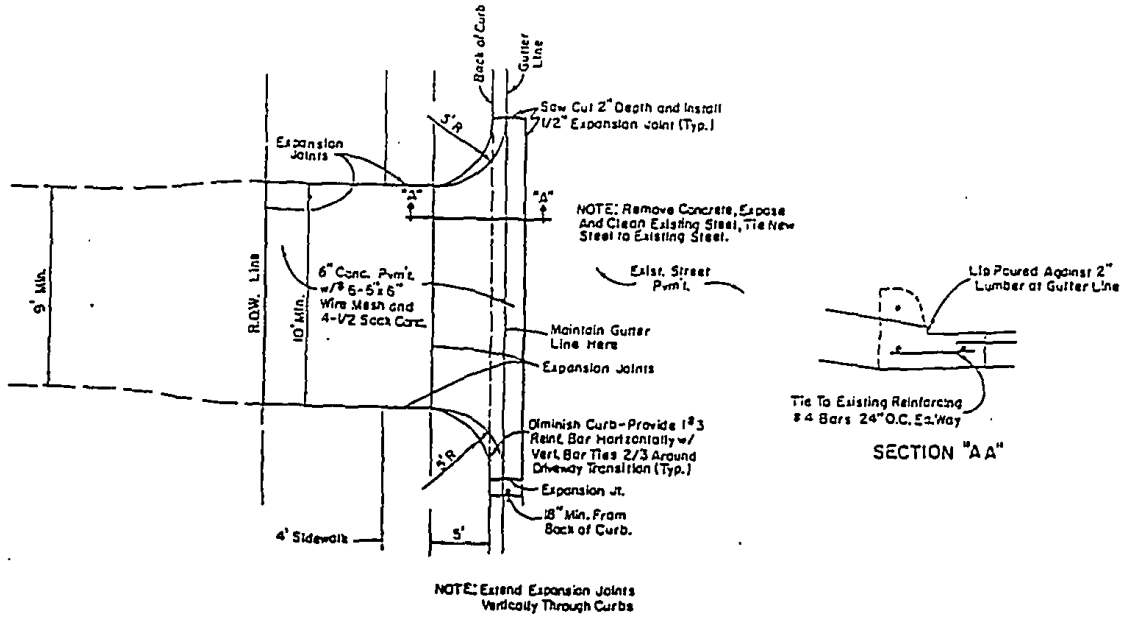
CONCRETE DRIVEWAY DETAIL N.T.S.
